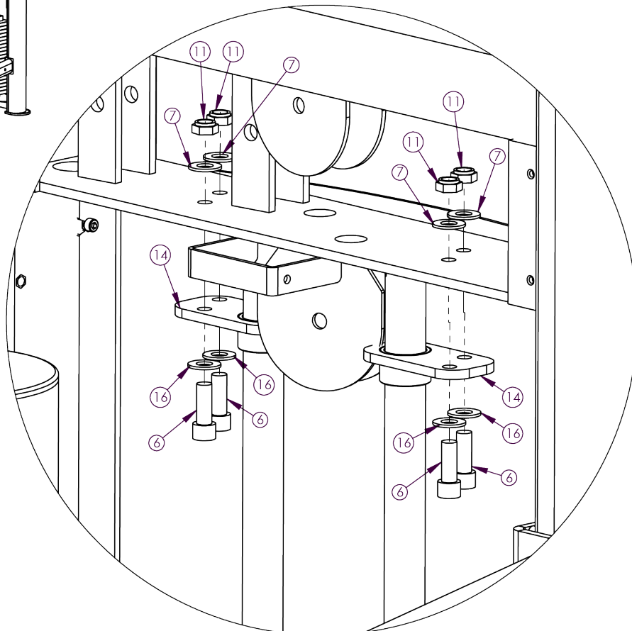
DETAIL K SCALE 1 : 3
