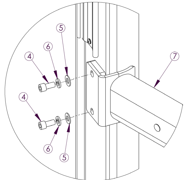
DETAIL E SCALE 1 : 5
